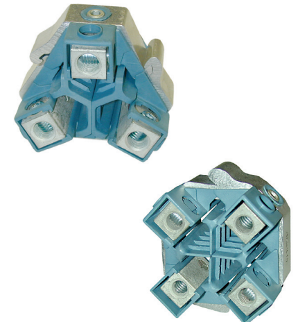
Ring Connector with Hexagon Socket Screw for 3- and 4-Core Cables
